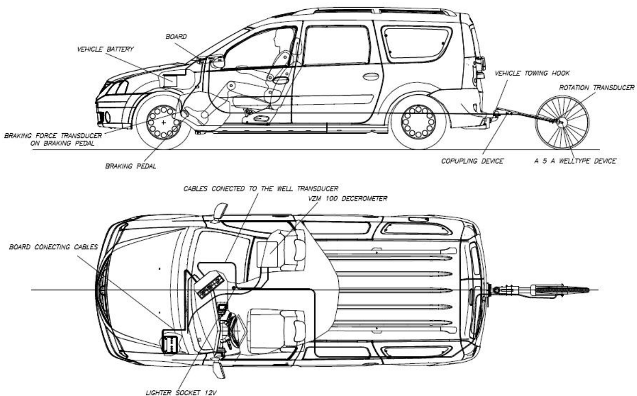
Figure 5. Principle scheme of a car endowed with the 5 th wheel
