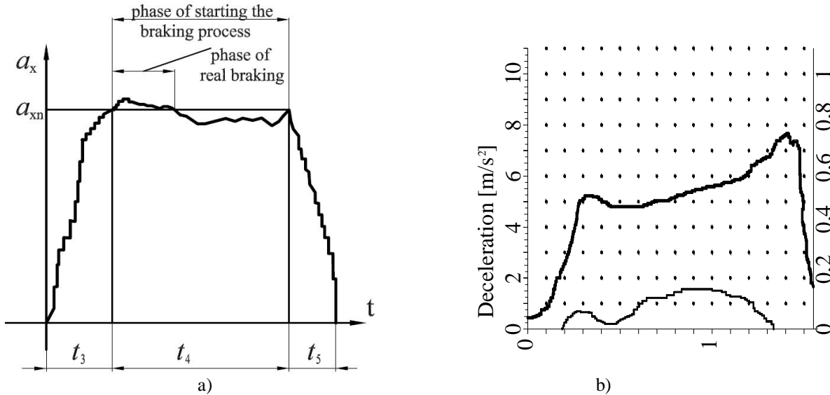
Figure 4 Diagram of braking without ABS: a)- phase of starting the braking process; b)- phase of real braking
